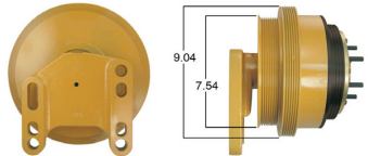
Part #99334 Caterpillar-C15 ACERT, C16 ACERT
