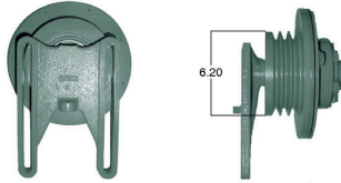
Part #91024 9.5" Friction Plate
