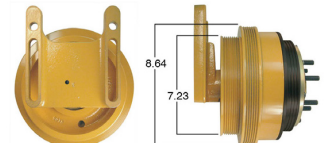
Part #99346 Caterpillar-C15 ACERT, C16 ACERT
